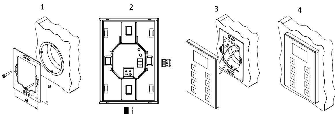
Figure 2 TMD-Display One. Installation Process.
