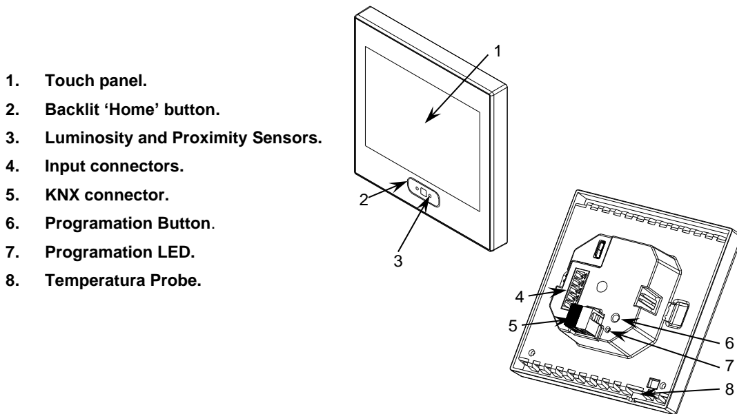
Figure 1. Schematic diagram Z35.
