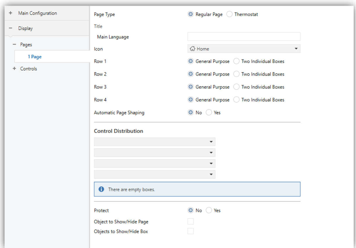
Figure 90. Regular page – Configuration (Vertical Z40).
